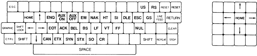
Figure 7. Characters with Control Key Depressed
